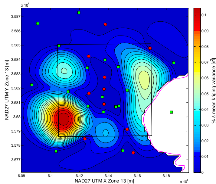
Figure 2-11. Change in mean kriging variance over WIPP LWB due to one additional well
