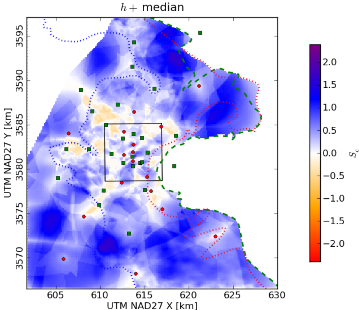
Figure 5-6. Combined scaled results for case 4, using median \Delta kriging variance, median \Delta triangle shape metric, and correlation between modeled head and \log_{10} particle travel time.
