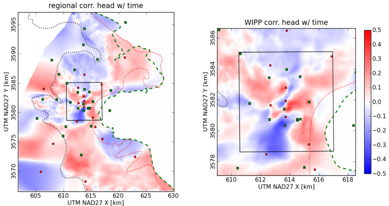
Figure 4-8. Correlation coefficient between model-predicted heads and \log_{10} (travel time) to WIPP LWB. Plot on right contains same data plotted on left.
