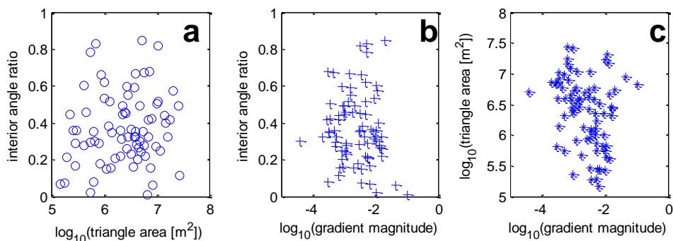
Figure 3-6. Scatter plots of relationships between different triangle metrics for 2007 Culebra well network.
