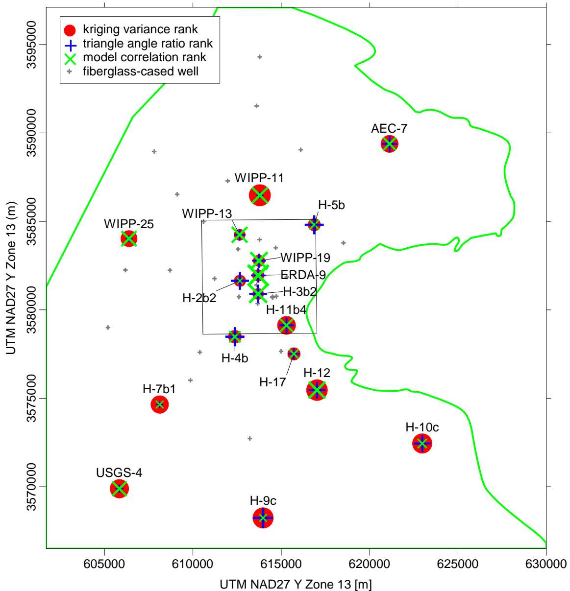
Figure 5-7. Composite plot of steel-cased well rankings from previous sections. Large symbols correspond to greater relative importance for each of the three measures.
