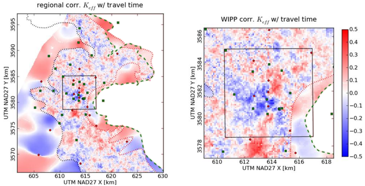
Figure 4-5. Correlation coefficient between \log_{10}(K_{eff}) and \log_{10} travel time to WIPP LWB. Steel-cased wells are red circles; fiberglass-cased wells are green squares. Salado dissolution and Rustler halite margins are indicated with dashed lines. Plot on right contains same data plotted on left.
