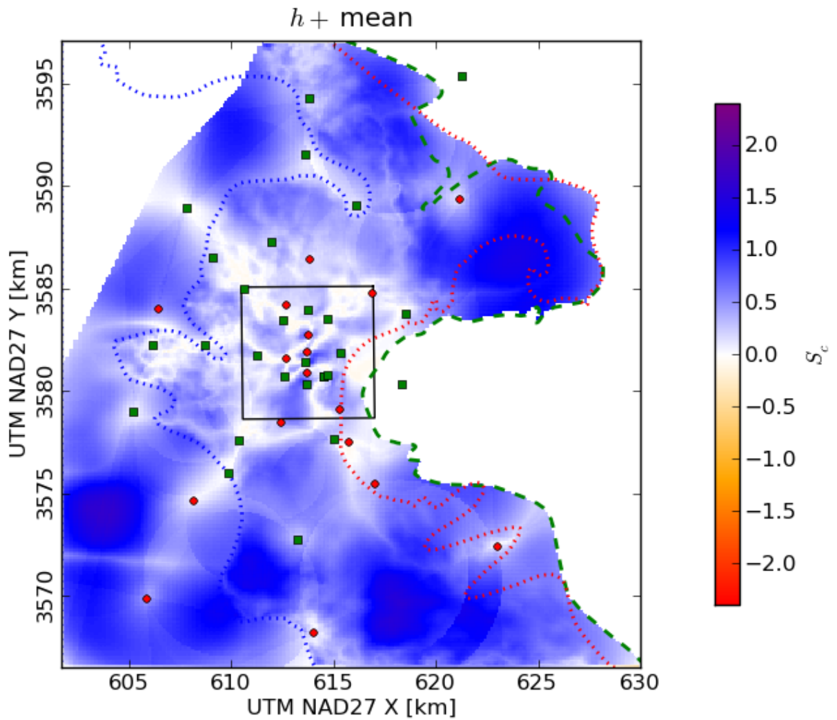
Figure 5-5. Combined scaled results for case 3, using mean \Delta kriging variance, mean \Delta triangle shape metric, and correlation between modeled head and \log_{10} particle travel time.
