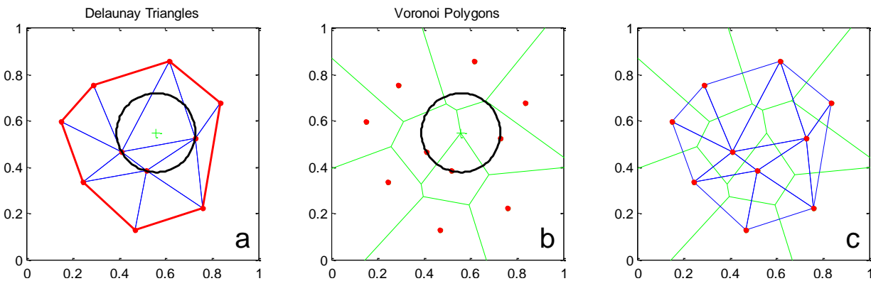
Figure 3-2. Delaunay triangles and Voronoi polygons for 10 randomly located points (red symbols). Black circle with green center used to illustrate the relationship between triangles (a) and polygons (b). Red lines indicate the convex hull, (c) shows both sets of polygons together.
