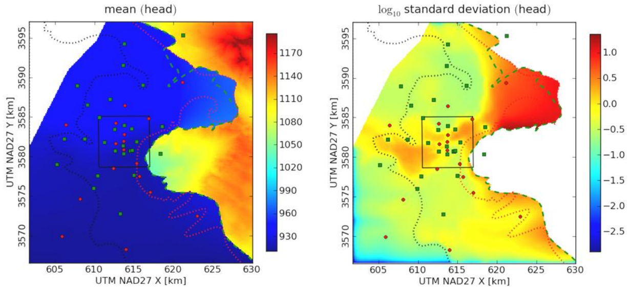
Figure 4-7. Mean and \log_{10} standard deviation of model-simulated head across all 100 realizations
