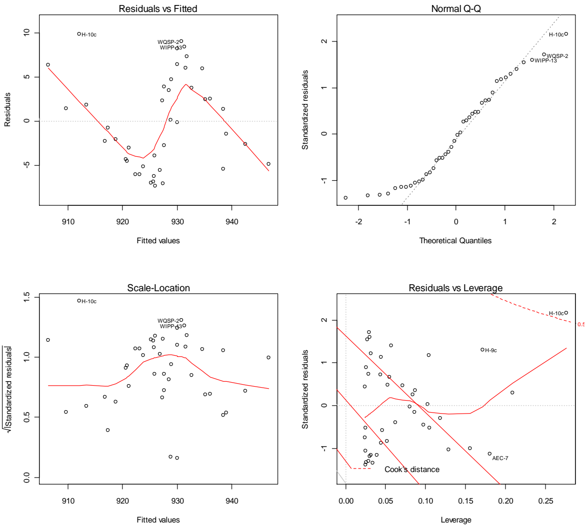
Figure 2-3. Statistics of linear surface (Equation 1) fit to May 2007 freshwater heads
