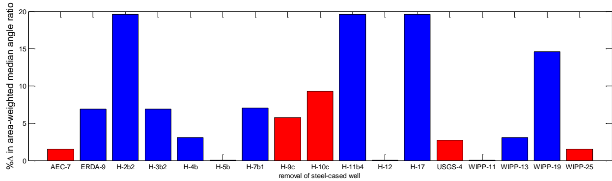
Figure 3-13. Change in median area-weighted angle ratio upon removal of each steel well from monitoring network (no SNL-6 or SNL-15).
