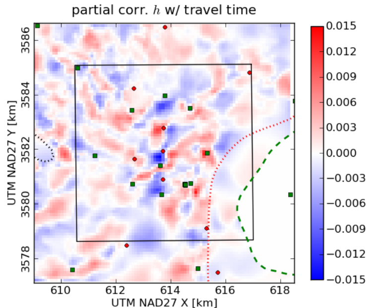
Figure 4-9. Partial correlation coefficient between model-predicted heads and \log_{10} (travel time) to WIPP LWB.
