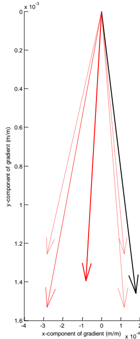
Figure 2-2. Comparison of gradient vectors corresponding to best-fit planes through 2003 (black) and 2007 (red) data. Red dotted lines correspond to estimated gradient \pm gradient standard error.
