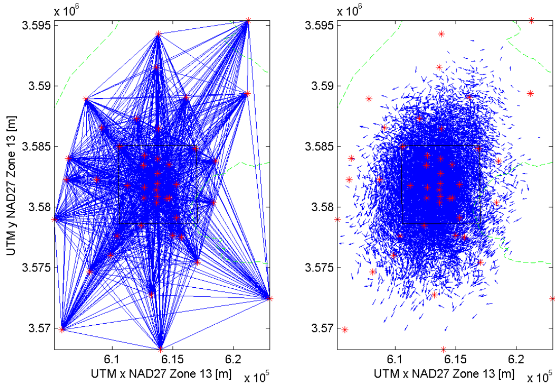
Figure 3-1. All possible triangles (left) and corresponding gradient vectors (right) for May 2007 Culebra monitoring network (as was used in the three-point estimator approach from first revision of this report). Vectors are \log_{10} length scaled; tails of vectors are anchored at the center of their triangle.
