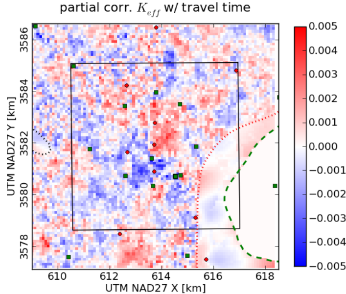
Figure 4-6. Partial correlation between \log_{10}(K_{eff}) and \log_{10}(\text{travel time}) to WIPP LWB
