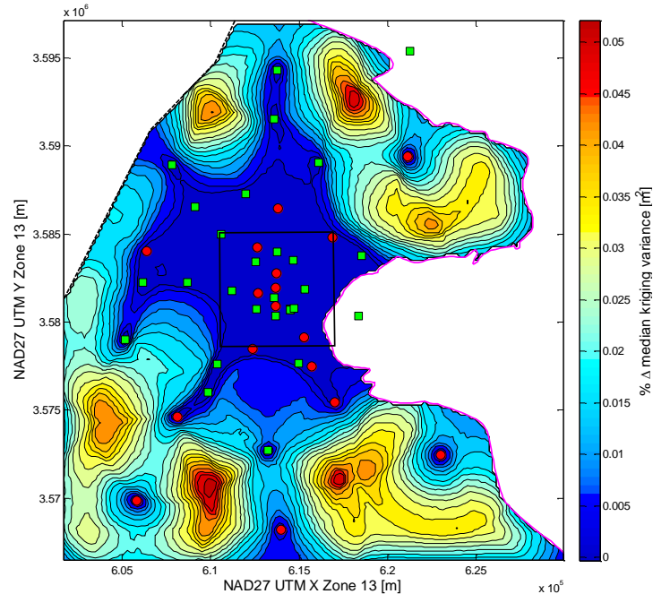
Figure 2-9. Percent decrease in median kriging variance over model domain due to one additional well
