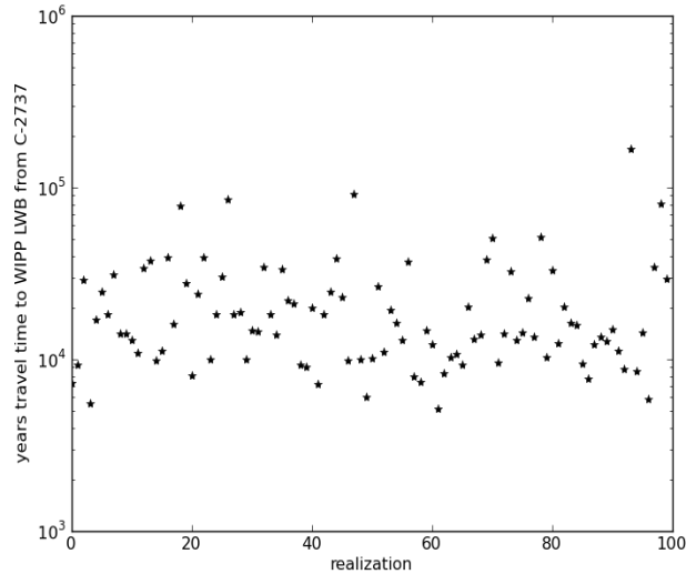
Figure 4-2. Travel times to WIPP LWB for conservative particle (non-dispersive, reactive, with no decay) for 100 realizations used in correlation analysis
