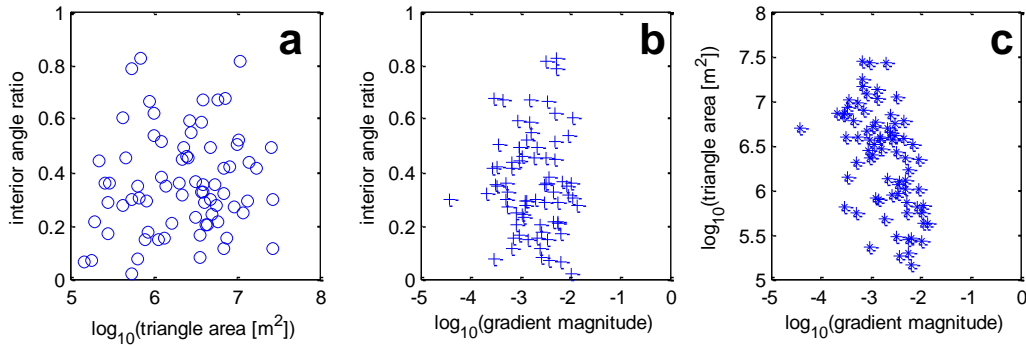
Figure 3-9. Scatter plots of relationships between different triangle metrics for 2007 network without SNL-6 and SNL-15.
