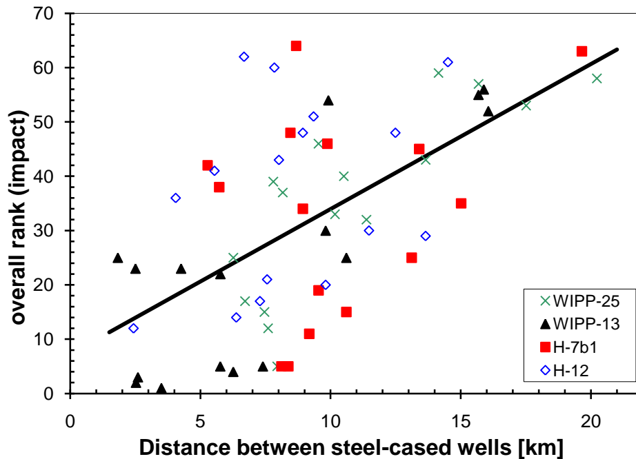
Figure 2-17. Rank and distance between wells for removal of pairs of steel-cased wells, averaging effects across the entire model domain ( R^2=0.35 for linear fit). High numerical rank indicates a large impact on the model-wide kriging variance.
