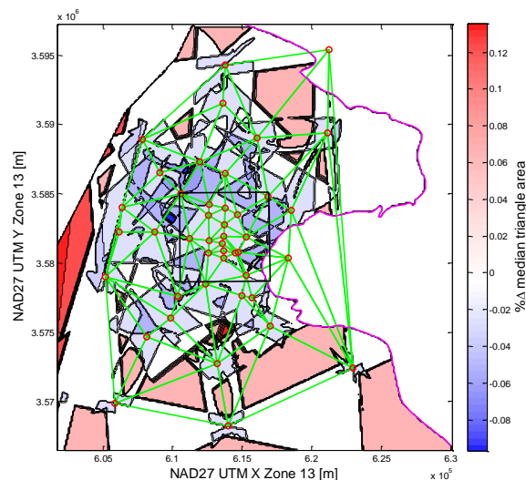
Figure 3-11. Increase (red) or decrease (blue) in median triangle area, due to including one additional well
