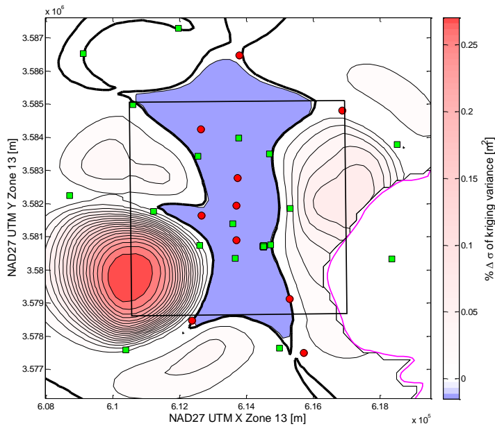
Figure 2-13. Change in standard deviation of kriging variance over WIPP LWB due to one additional well
