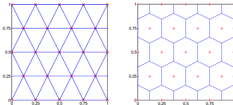
Figure 3-4. Delaunay triangles and Voronoi polygons for symmetric triangular mesh
