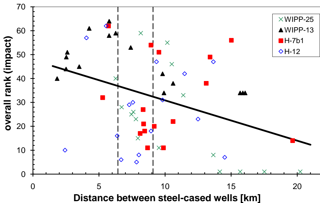
Figure 2-18. Rank and distance between pairs of steel-cased wells, considering WIPP LWB ( R^2=0.14 for linear fit). Vertical dashed lines represent the min (6.4 km) and max (9.1 km) distances across the LWB. High numerical rank indicates a large impact on the kriging variance inside the WIPP LWB.
