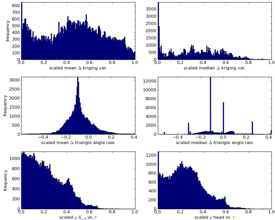
Figure 5-2. Histograms of each component of S_c , after applying scaling
