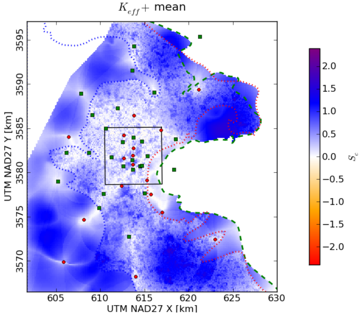
Figure 5-3. Combined scaled results for case 1, using mean \Delta kriging variance, mean \Delta triangle shape metric, and correlation between K_{eff} and \log_{10} particle travel time. Fiberglass-cased wells are green squares, steel-cased wells are red circles; Salado dissolution and Rustler halite margins are dashed lines; WIPP LWB is black square.
