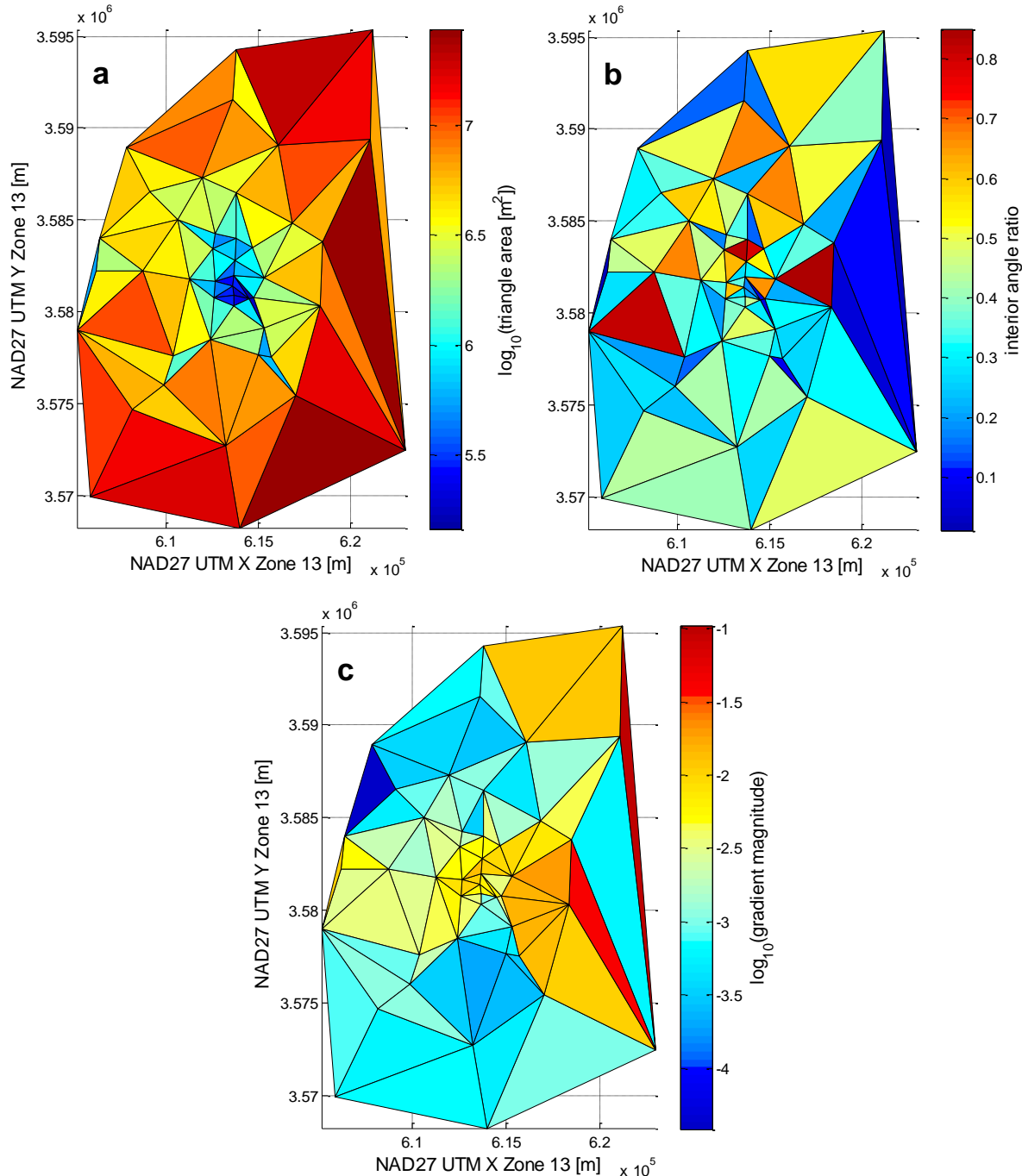
Figure 3-5. Distribution of geometry metrics for 2007 Culebra well network: (a) area of triangle, (b) angle ratio, and (c) May 2007 freshwater head gradient magnitude.
