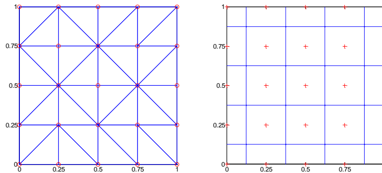
Figure 3-3. Delaunay triangles and Voronoi polygons for symmetric square grid; note ambiguity in triangles
