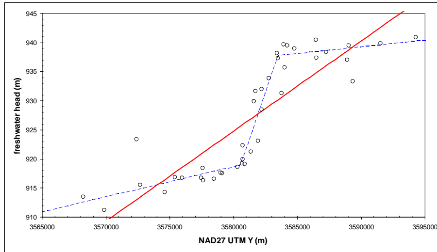
Figure 2-1. Projection of freshwater heads (circles), piecewise linear trend (blue dashed line), and best-fit linear trend (red line) onto y-head plane at x-midpoint of MODFLOW model domain.
