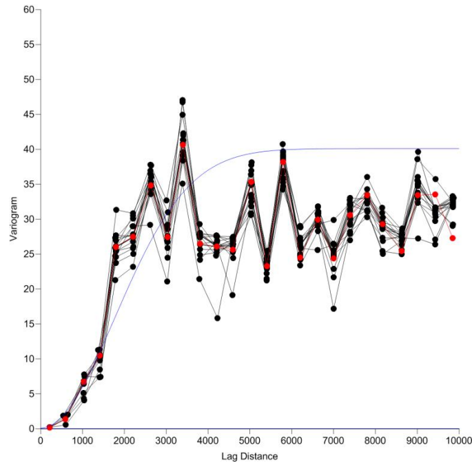
Figure 2-6. Experimental variograms after removing a steel-cased well (variogram for all wells shown in red). Residuals are re-computed based on the best-fit linear trend for each new set of wells and the variogram is re-computed for each new set of residuals.
