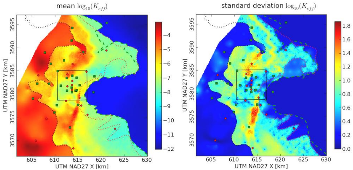
Figure 4-4. Mean and standard deviation of \log_{10}(K_{eff}) across all 100 realizations
