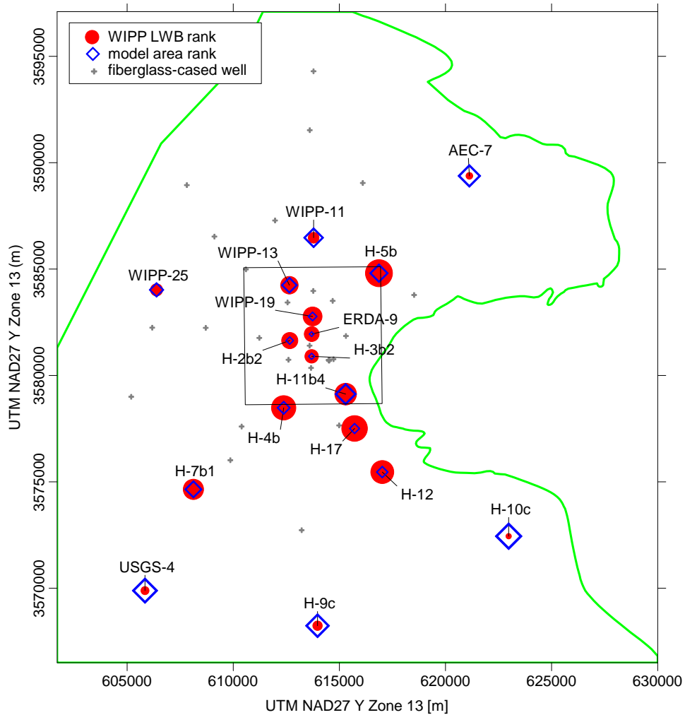
Figure 2-15. Steel-cased wells ranked by effect of removal on kriging variance; symbol sizes are proportional to overall rank (and therefore importance), data in Table 2-3 and Table 2-4. MODFLOW active model domain delineated in green, WIPP LWB is black square.
