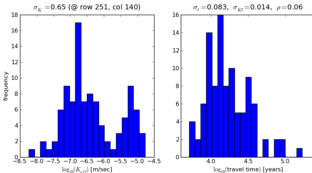
Figure 4-1. Example histograms of a model parameter ( \log_{10}(K_{eff}) ) at a particular cell and model prediction ( \log_{10}(\text{travel time to WIPP LWB}) ) across all 100 realizations.
