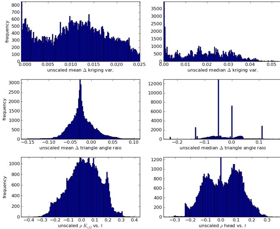
Figure 5-1. Histograms of each component of S_c , before applying scaling.
