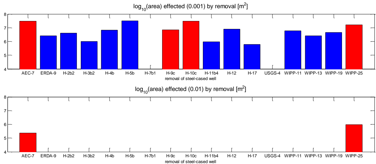
Figure 3-14. Area affected ( \Delta gradient magnitude \geq 0.01 ) by removal of steel well
