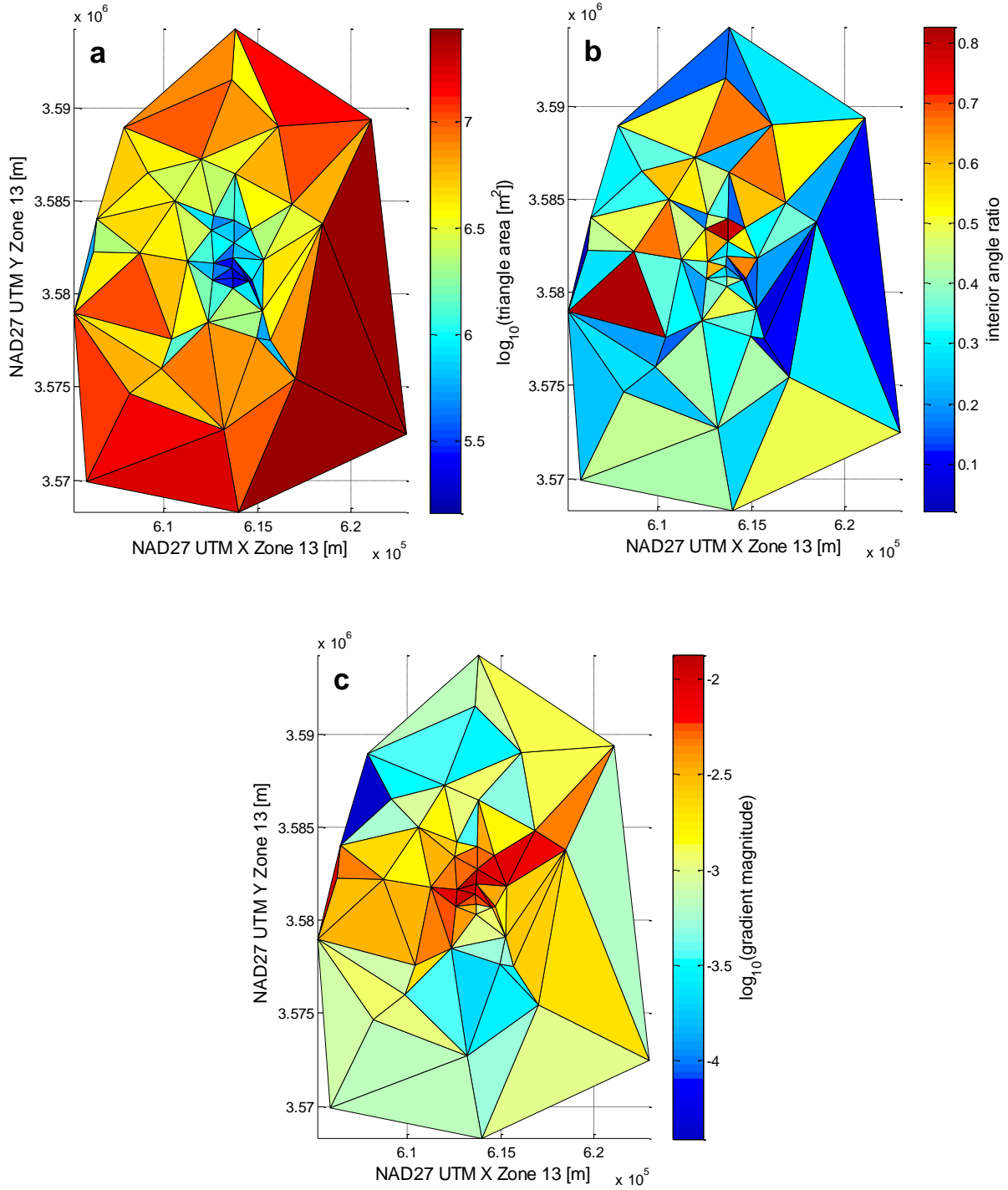
Figure 3-8. Distribution of triangle geometry metrics: (a) triangle size, (b) interior angle ratio, and (c) May 2007 freshwater head gradient magnitude for 2007 network without SNL-6 and SNL-15
