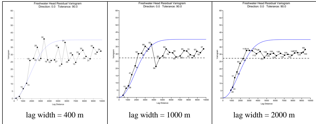
Figure 2-5. Experimental variograms (points) and best-fit Gaussian model variogram (lines) for three different lag widths. NB: there is a factor-of-three difference in definition of variograms between Surfer and GSLIB (multiply lag by 3.0).
