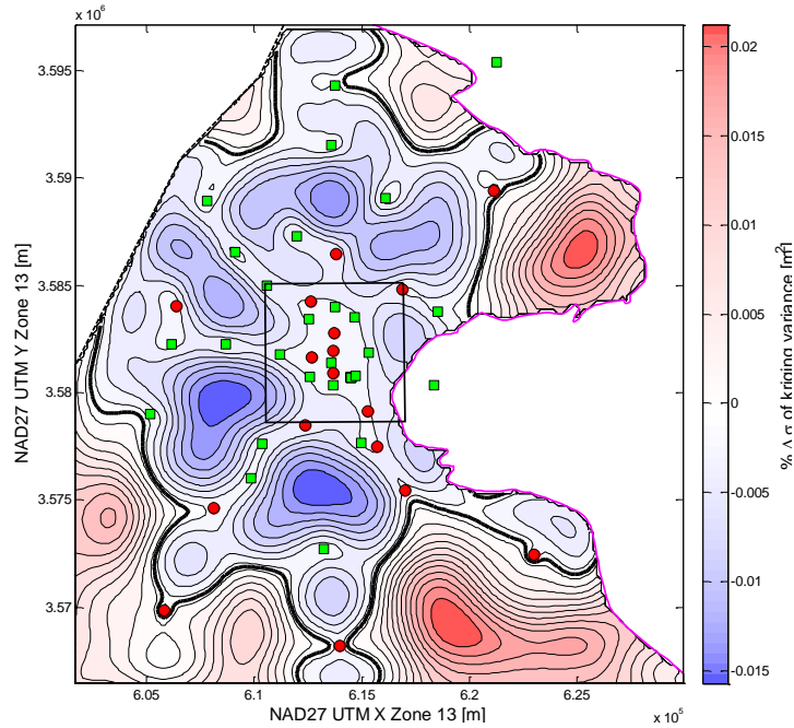
Figure 2-10. Percent change in standard deviation of kriging variance over model domain due to one additional well; heavy black line is zero contour.
