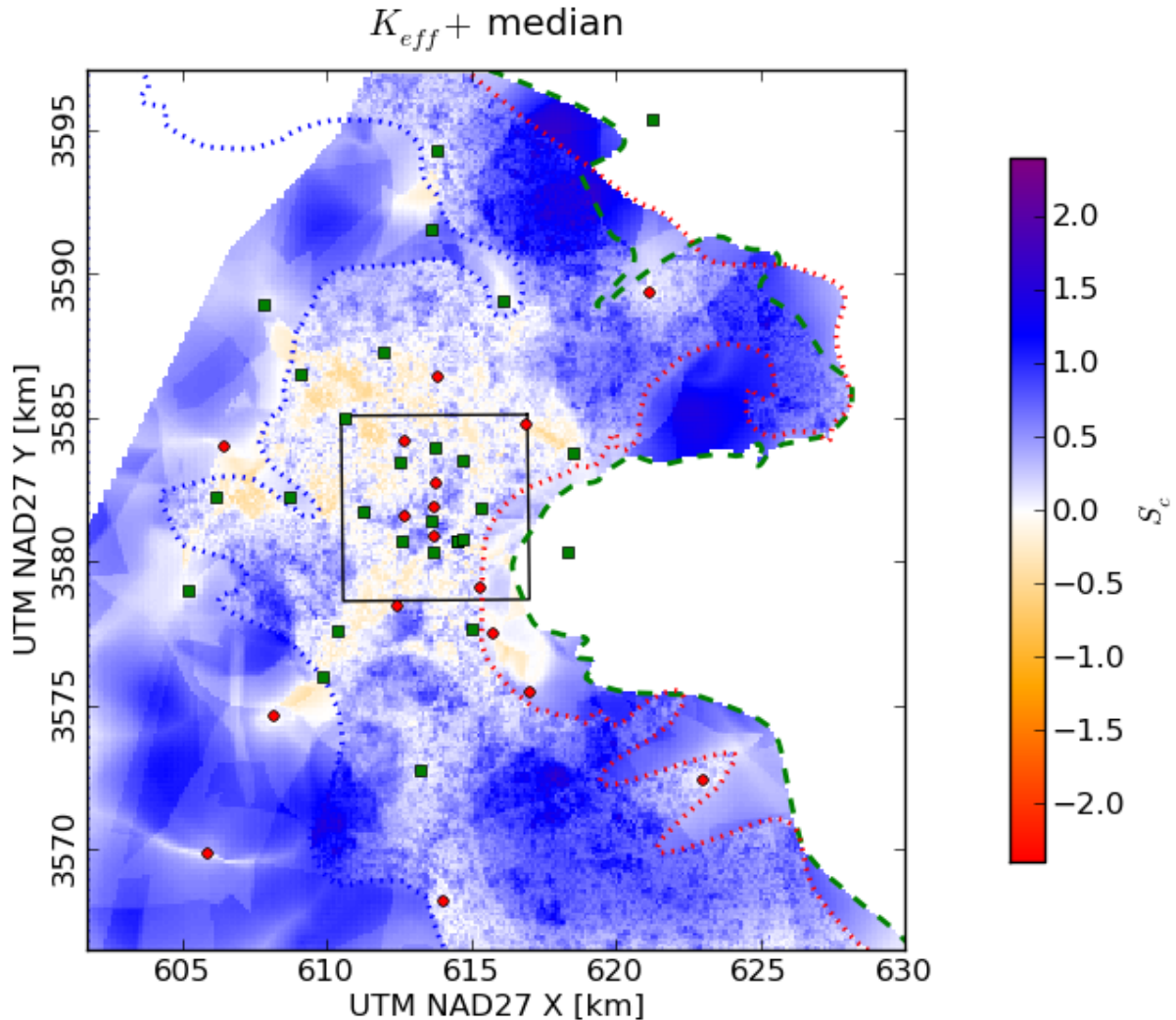
Figure 5-4. Combined scaled results for case 2, using median \Delta kriging variance, median \Delta triangle shape metric, and correlation between K_{eff} and \log_{10} particle travel time.
