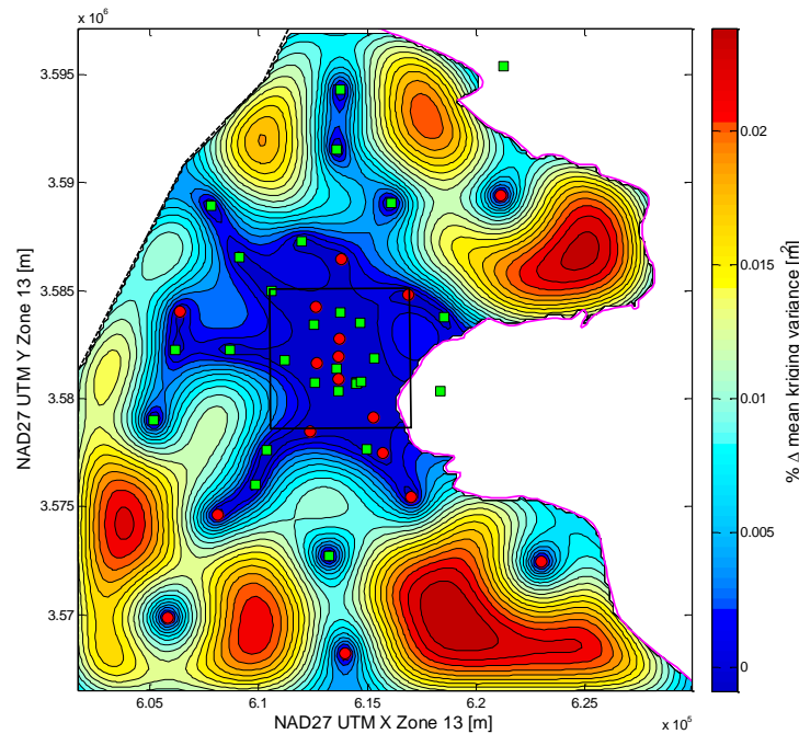
Figure 2-8. Percent decrease in mean kriging variance over model domain due to one additional well
