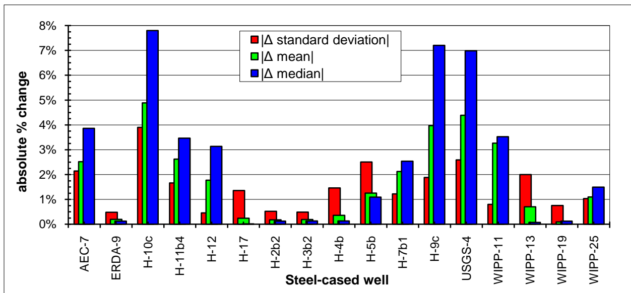
Figure 2-14. Change in estimation variance averaged across entire model domain (data from Table 2-3)
