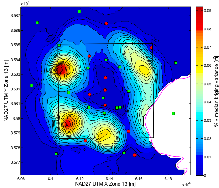
Figure 2-12. Change in median kriging variance over WIPP LWB due to one additional well
