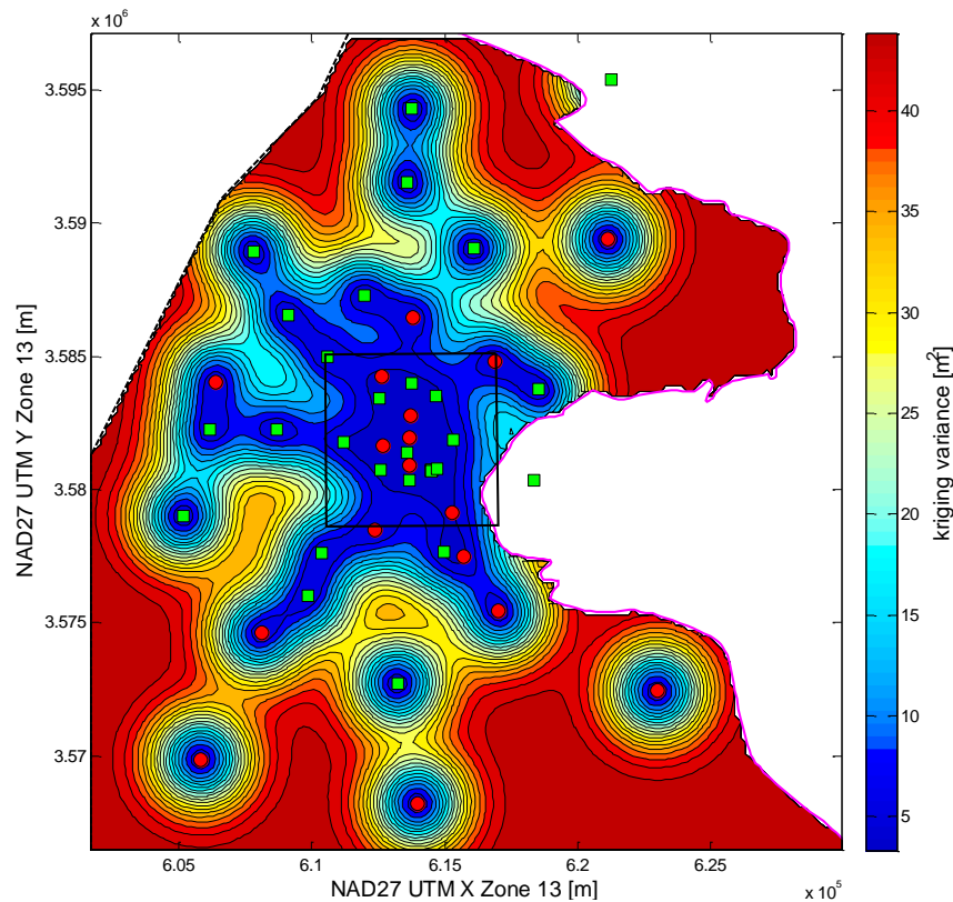
Figure 2-7. Kriging estimation variance for freshwater head residuals. Steel-cased wells are red circles, fiberglass wells are green squares, WIPP LWB is solid black line.
