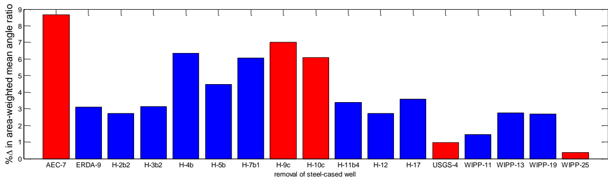
Figure 3-12. Change in mean area-weighted angle ratio (averaged over model domain) upon removal of each steel well from monitoring network (no SNL-6 or SNL-15). Red bars are wells located on convex hull.
