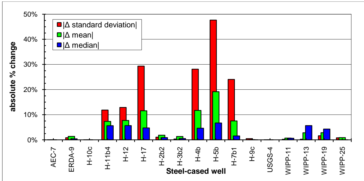
Figure 2-16. Change in estimation variance averaged across WIPP LWB, data in Table 2-4
