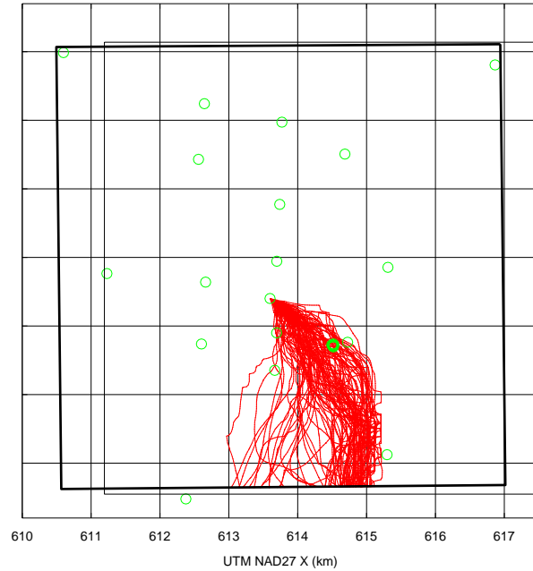
Figure 4-3. Marked water particle tracks from each of the 100 realizations; each track goes from the release point at C-2737 to the WIPP LWB (heavy black square). Green circles are Culebra monitoring wells.
