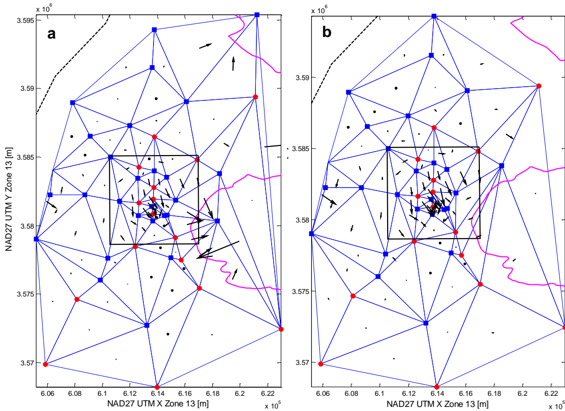
Figure 3-7. Delaunay triangles for 2007 Culebra network (a) with and (b) without SNL-6 and SNL-15. Gradient plotted as arrows (tails starting at center of triangle); length of arrow is proportional to magnitude gradient, arrow orientation indicates groundwater flow direction. WIPP LWB (black solid), M2/H2 - M3/H3 composite Rustler halite margins (magenta), and no-flow (black dashed) boundaries shown.
